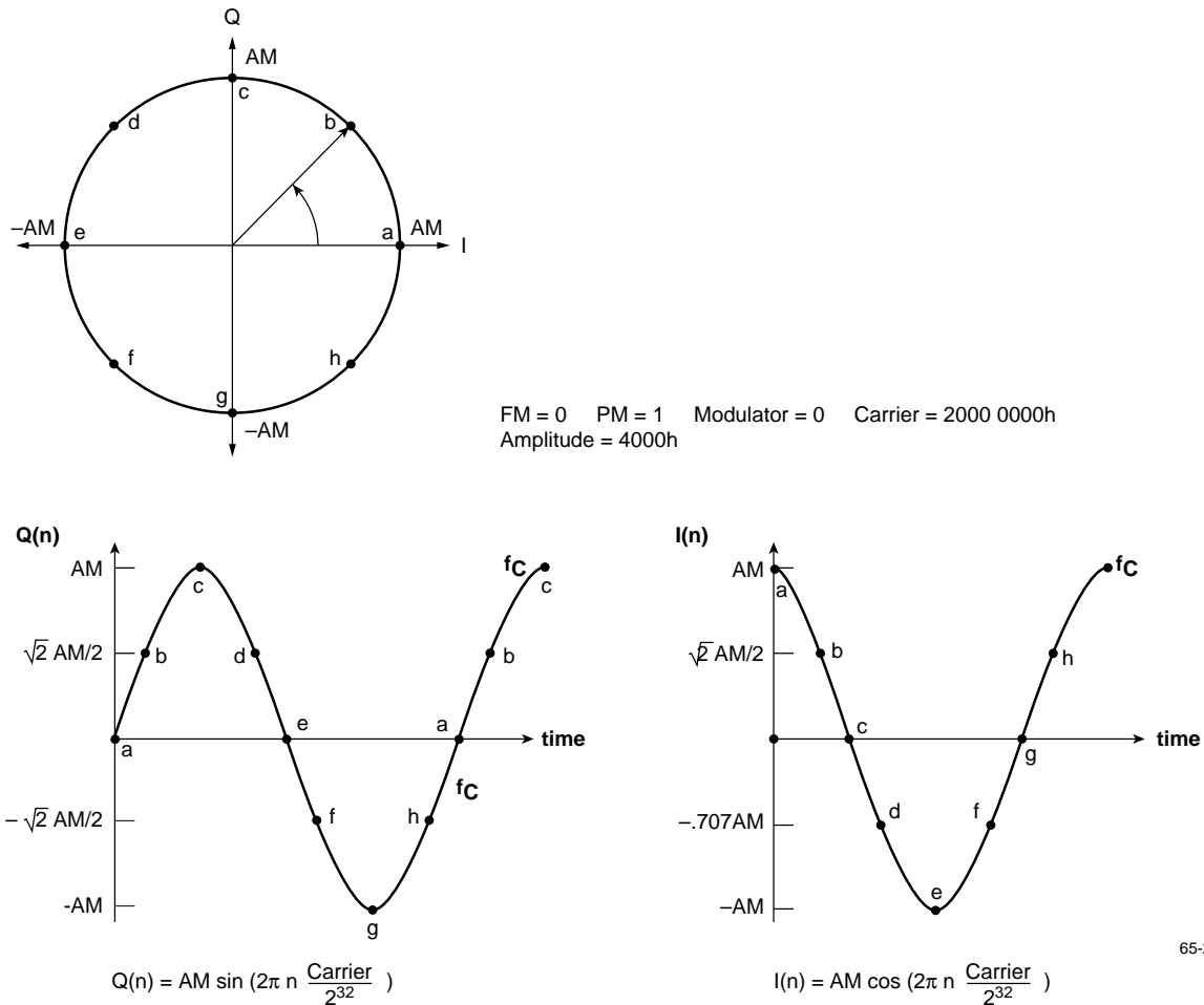
Figure 4. Unmodulated Sinusoid Generation
