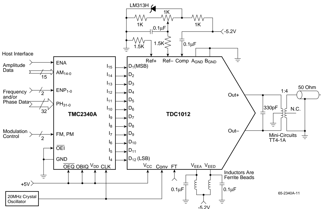
Figure 5. Frequency Synthesizer
